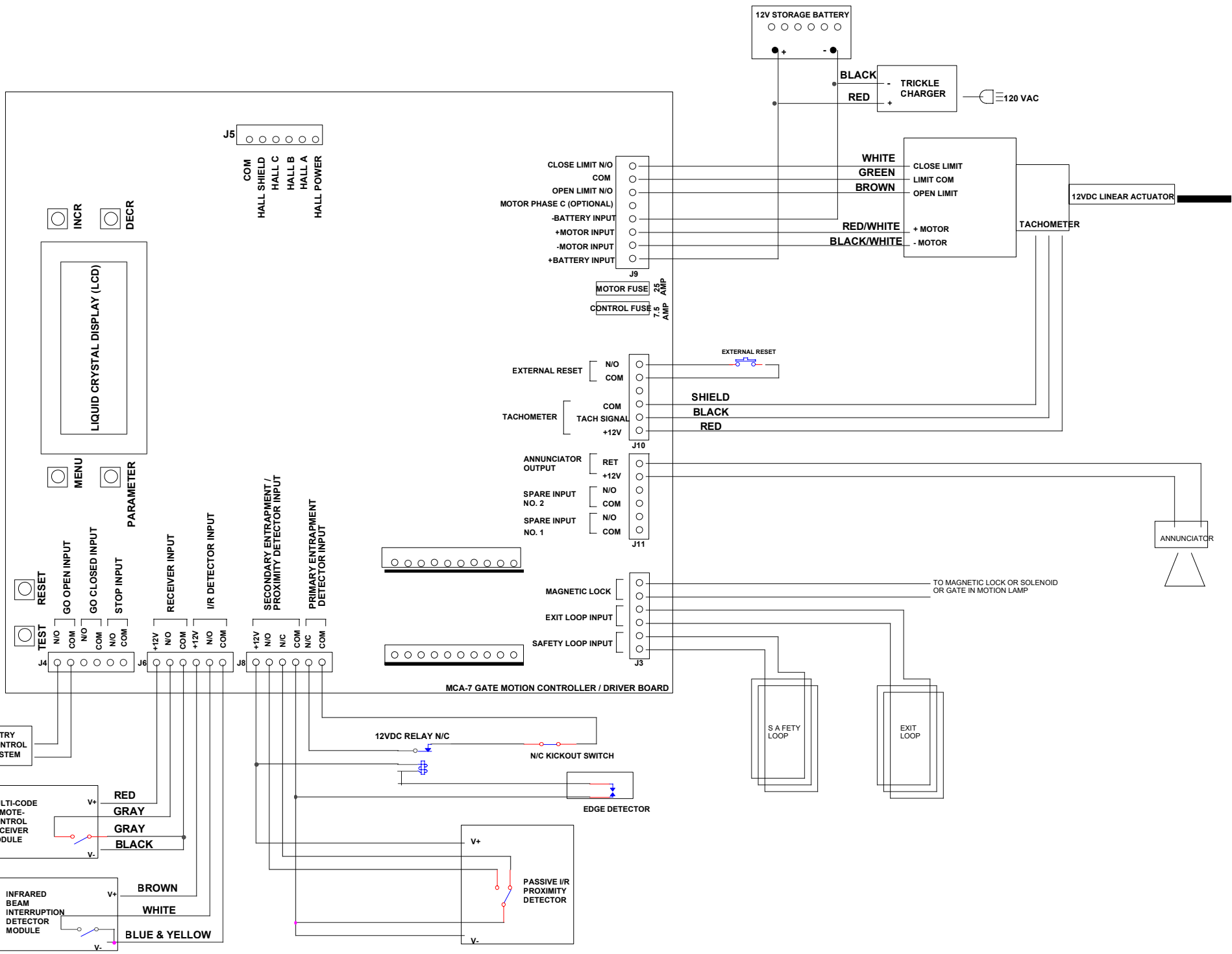
BLOCK DIAGRAM - MCA-7
